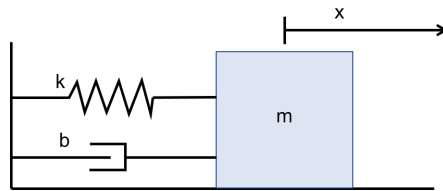
Figure 1: Mass-spring-damper system.
